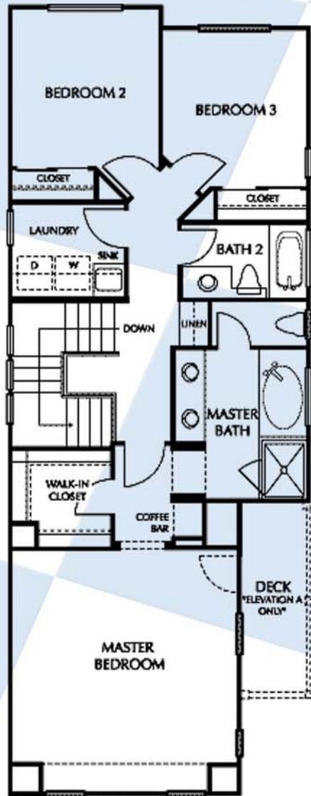
PLAN 1BR SECOND STORY
