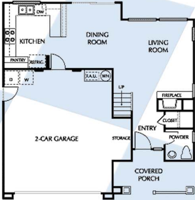
PLAN 3C FIRST FLOOR
